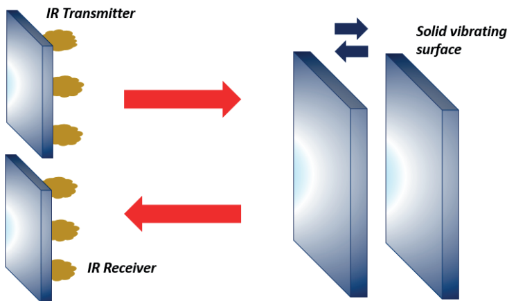
Figure 1. Proposed scheme of the IR receiver/transmitter from the designed smart sensor.
