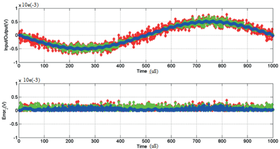
Figure 7. Experimental data analysis for the designed smart sensor
