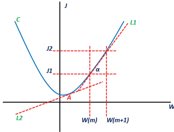
Figure 3. Geometric representation of the adaptive algorithm by LMS analysis.
